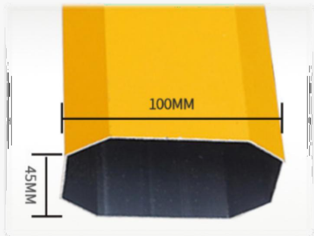
Octagonal pole
